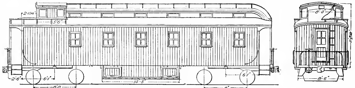
Fig. 165-166. BOARDING CAR. CHICAGO, BURLINGTON & QUINCY RAILROAD.
